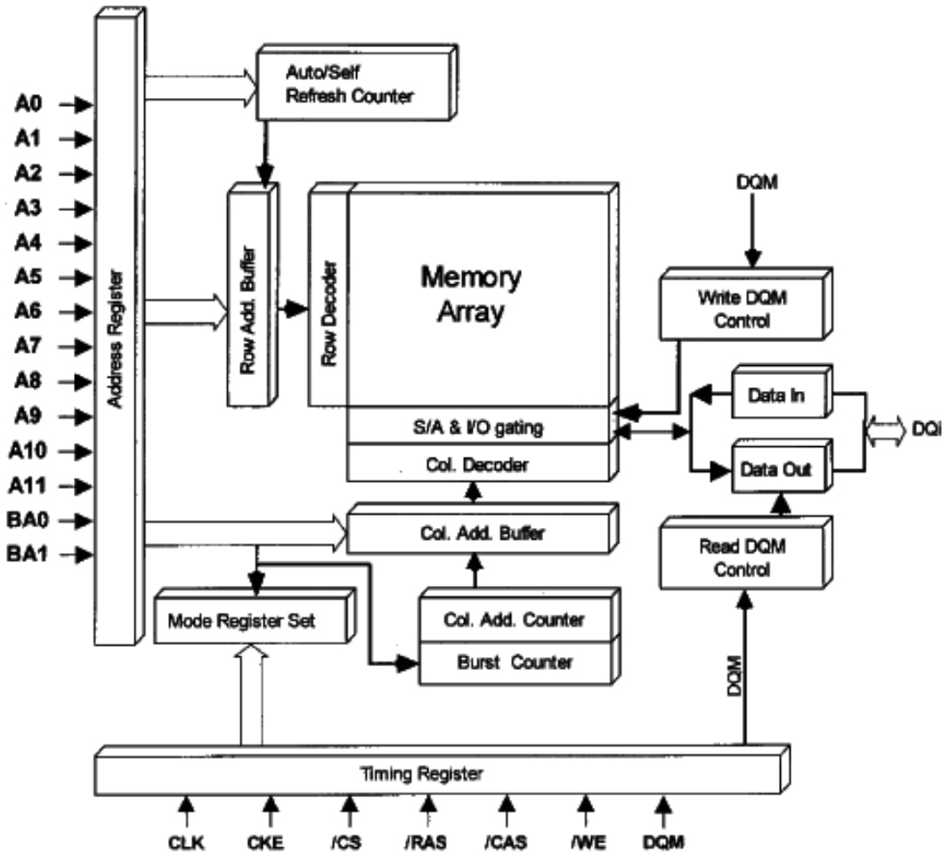
Internal IC diagram -V5888S HSOP
