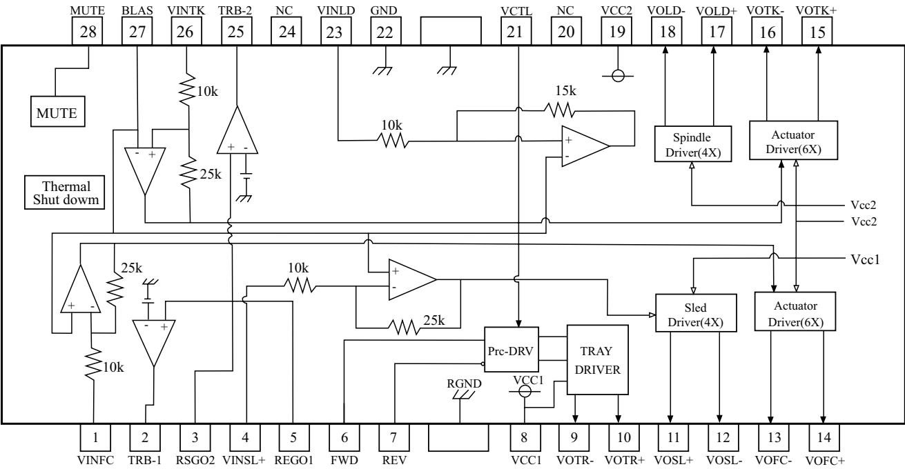
Internal IC diagram -V5888S HSOP
