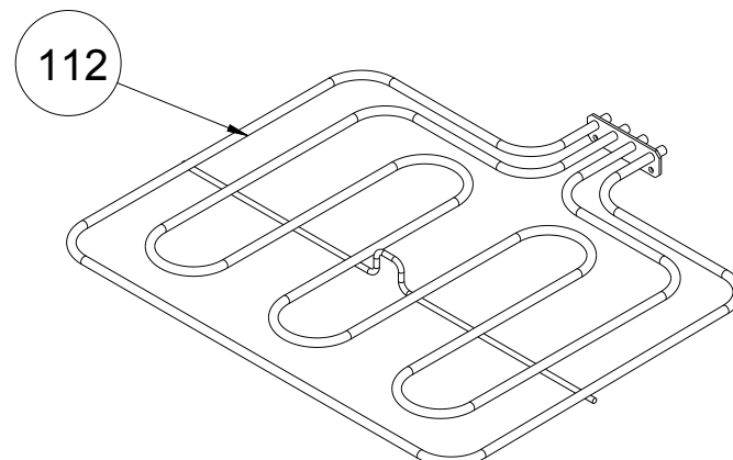
TOP AND GRILL HEATING ELEMENT (OPTIONAL)
