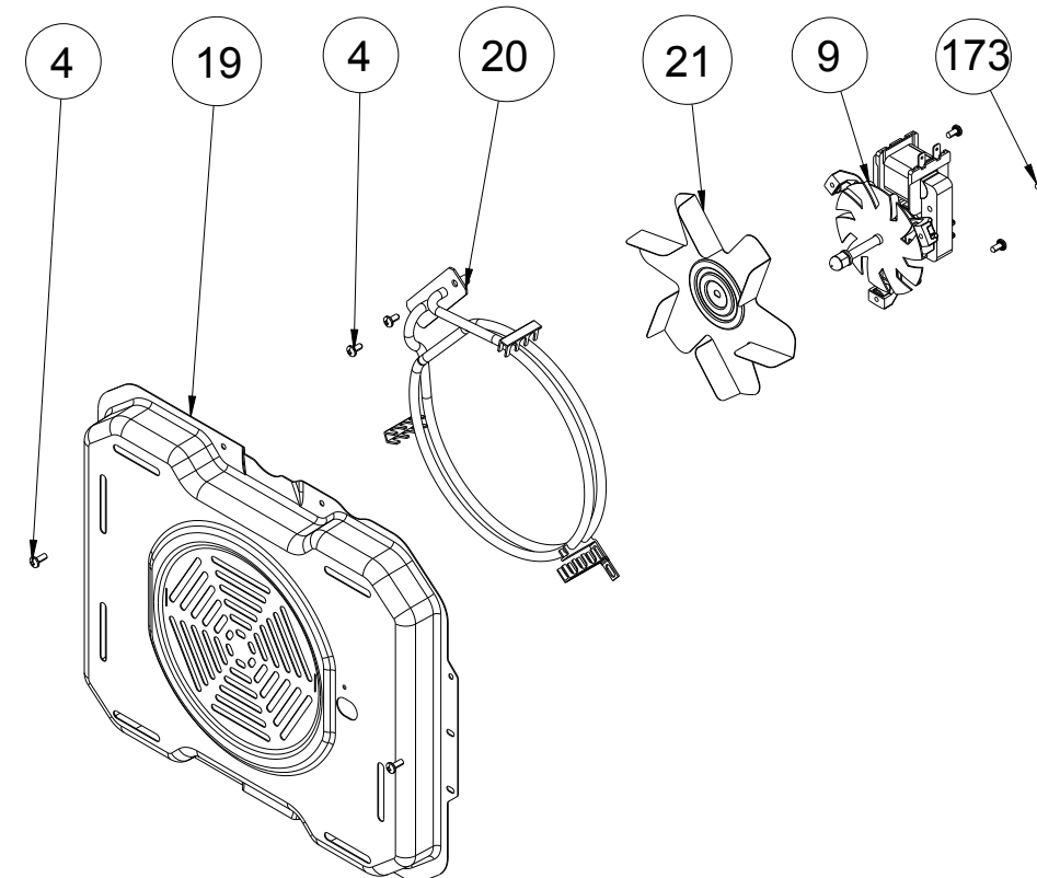
RING HEATING ELEMENT WITH FAN (OPTIONAL)
