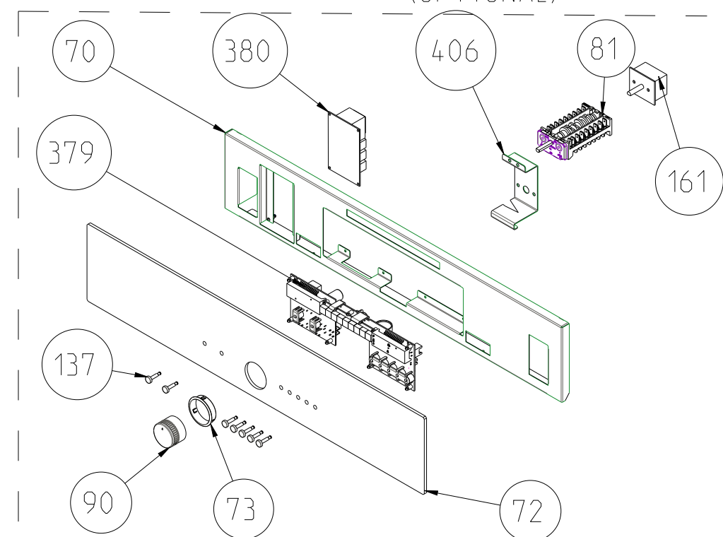
GLASS CONTROL PANELS WITH INOX ADD-ONS (OPTIONAL)
