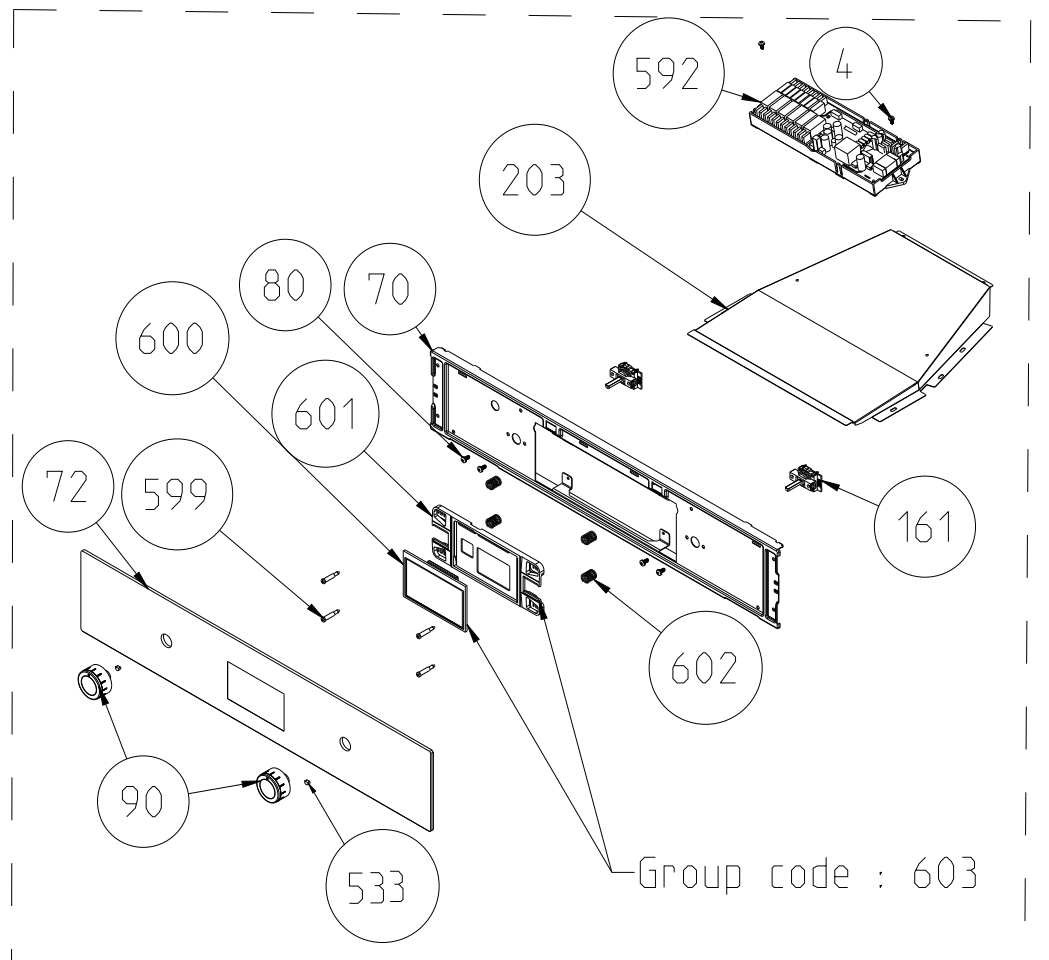
LCD SMART GLASS CONTROL PANEL ASSEMBLY (OPTIONAL)
