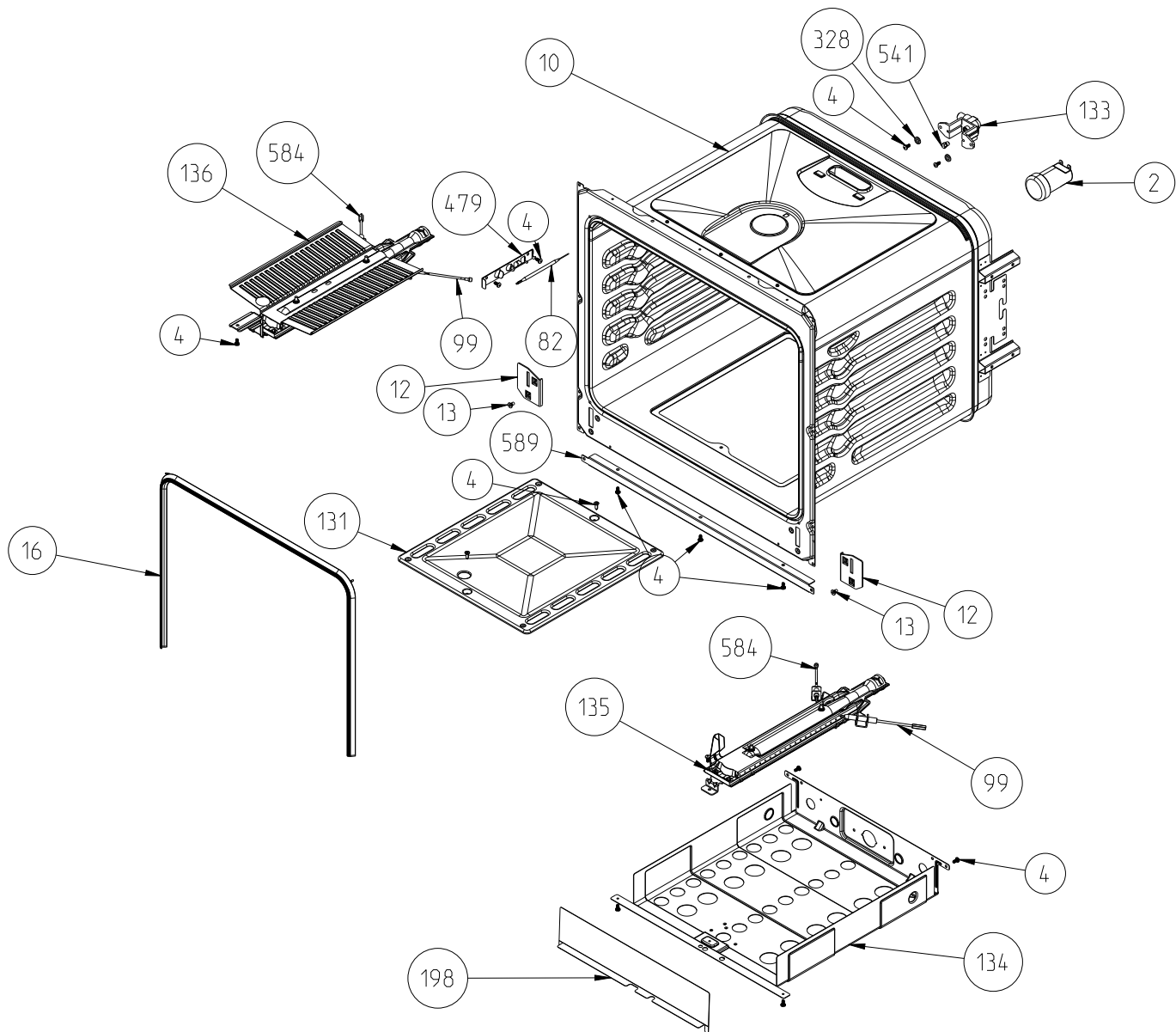
GAS OVEN GAS GRILL CAVITY ASSEMBLY
