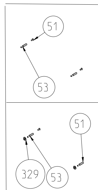
HANDLE ASSEMBLY GROUP (POSITION NO 49) (OPTIONAL)
