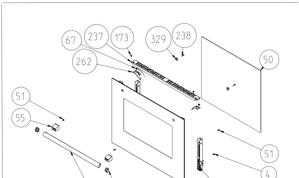
OVEN DOOR ASSEMBLY (OUTER & INNER) (POSITION NO 378)
