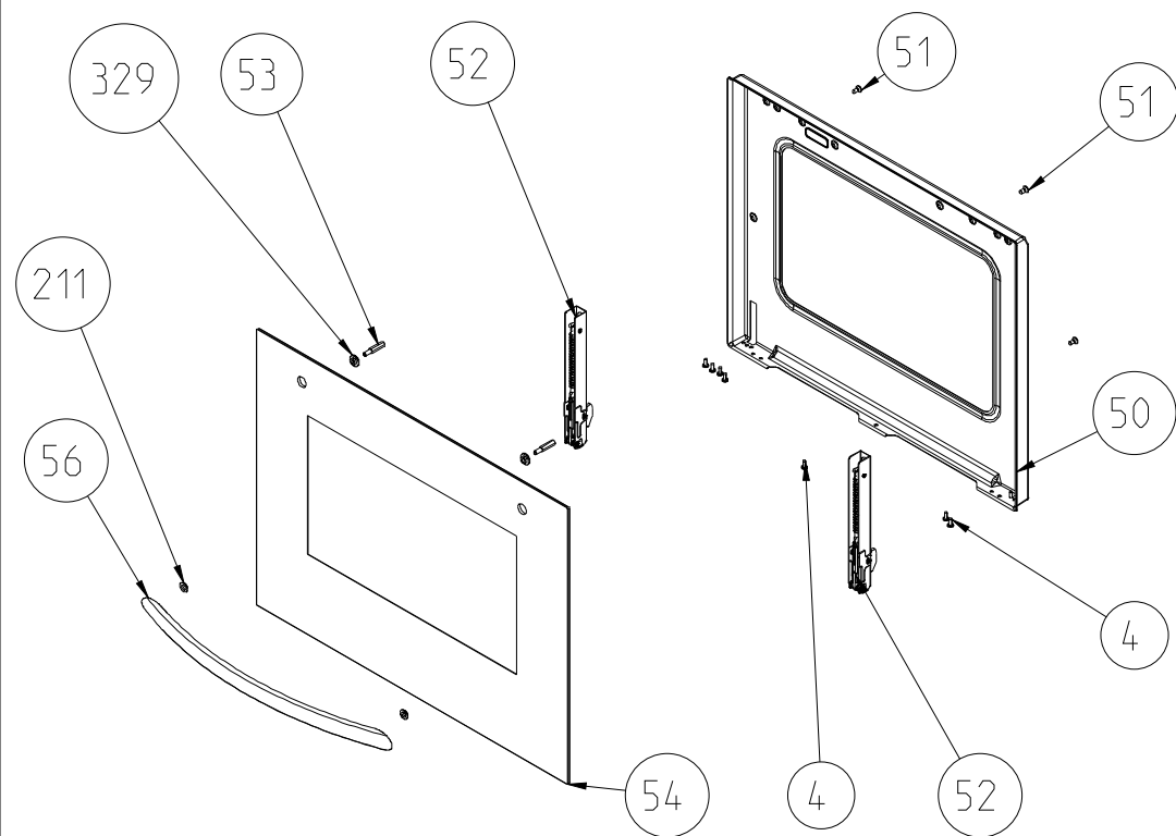
OVEN DOOR ASSEMBLY (OUTER & INNER) (POSITION NO 378)
